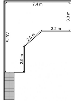
Mezzanine Level
